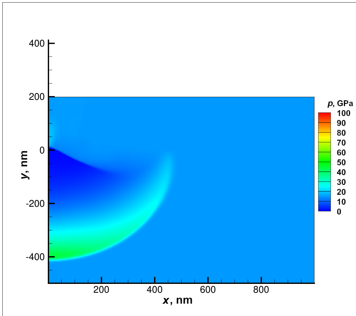
Figure 6. Pressure field at the same time instant t = 100 ps as in figure 5. Grid cell size equals 2 nm. This calculation has an important difference from the calculation in figure 5. The ratio of densities between vacuum and target substances has been increased a hundred times. Here it is equal to 10^{-4} . The results differ little. The only noticeable difference is the disappearance of the weak oblique shock wave, which is visible in figure 5.
