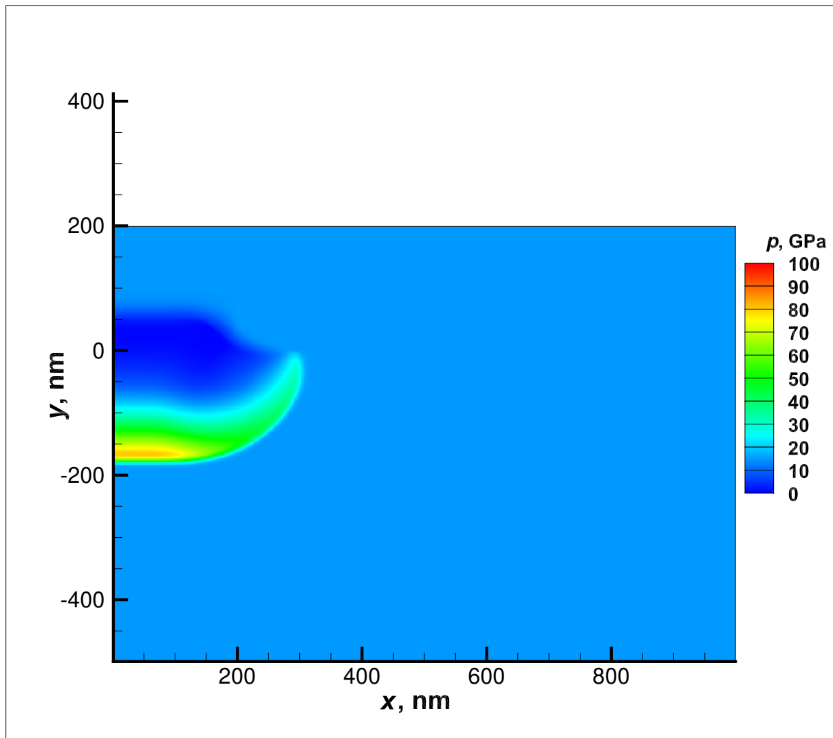
Figure 8. Pressure field at t = 30 ps. Grid cell size is 2 nm. The plane shock wave continues to propagate into the target thickness, compare with the situation at the time of 10 ps in figure 7. At the same time, lateral discharge waves are moving further along the front of the flat shock wave. We note a fairly strict limitation of the emission into vacuum (laser torch) by the size of the half-width of the laser beam R_L = 200 nm.
