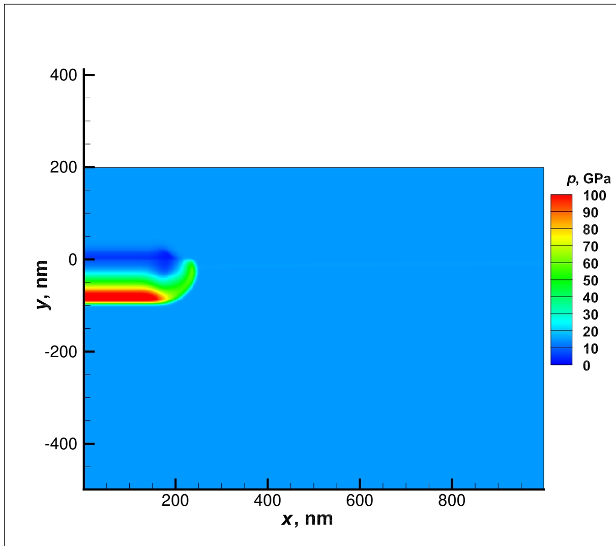
Figure 7. Pressure field of laser-induced flow in a volume target at the instant of 10 ps after a laser strike. Grid cell size is equal to 2 nm. The initial pressure in the rapid heating rectangle 3 in figure 3 was 2.6 Mbar. The ratio of vacuum densities to the target is 10^{-4} . Therefore, acoustic disturbances in vacuum have such a negligible amplitude that they are not visible on this pressure map, compare. with a weak oblique wave visible in figure 5 with a density ratio of 10^{-2} . Ahead, a quasi-flat shock wave runs into the thickness of the target. There are rounding side waves. The blue area refers to the discharge of the heated target material from rectangle 3 in figure 3 in the direction of vacuum.
