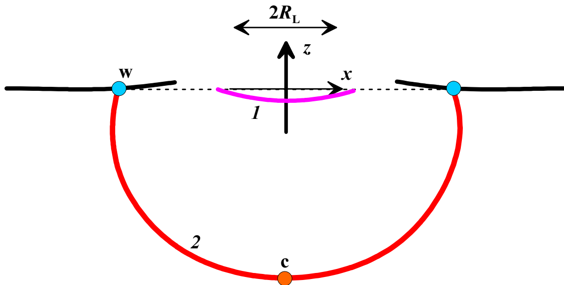
Figure 1. The scheme of action of an ultrashort laser pulse. The pulse creates a thin warmed up d_T -layer ( d_T \ll R_L ) at the surface. This layer is also a high-pressure layer at the initial stage. Decay of the high-pressure layer along the d'Alembert forms a quasi-plane characteristic 1 , propagating into the target volume. With a strong impact, a quasi-plane SW 1 runs ahead. At the propagation distances of this SW in depth of the order of the laser beam radius z_c \approx R_L a quasi-plane SW (front of SW 1 ) is transformed into a quasi-hemispherical SW (front SW 2 ). In this case, the attenuation of SW increases sharply due to spatial divergence. Due to the presence of a free boundary (the boundary of the target with vacuum), wave amplitude decreases from the point "c" to the point "w". At the "w" point, the slash line is adjacent to the border.
