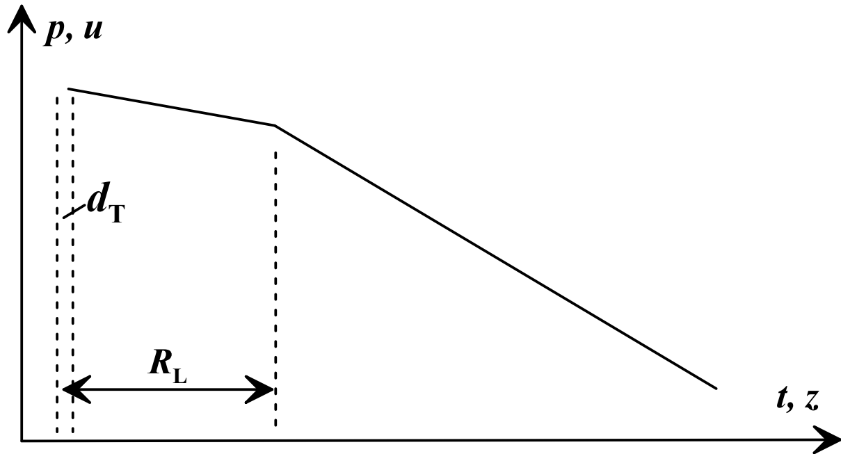
Figure 2. Changing the SW attenuation modes with a distance of z or a time of t . The values p, u are pressure and velocity values immediately behind the SW front at the central point “c” shown in figure 1. The mode change occurs at z \approx R_L or at times t_L \approx R_L/c_s .
