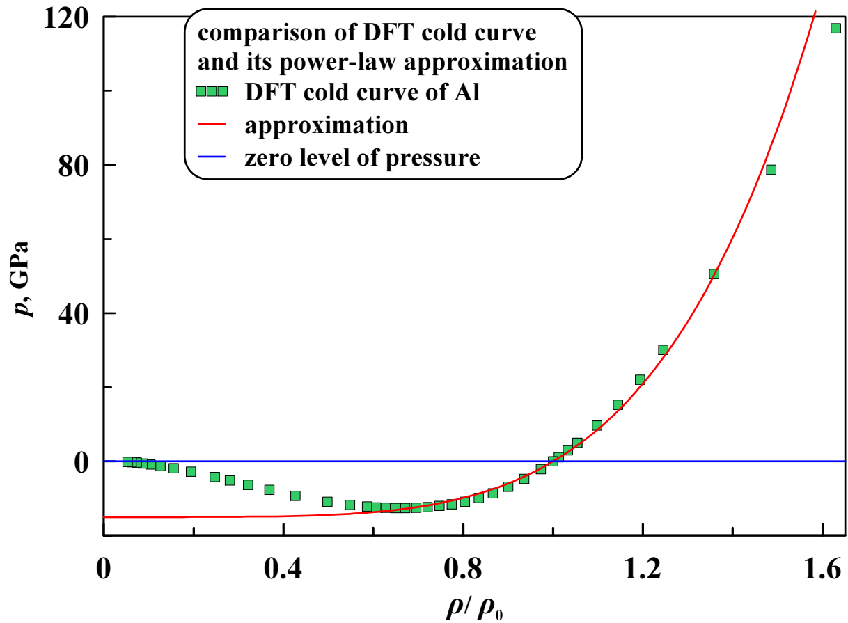
Figure 4. Equation of state of the target substance and approximation of this equation.
