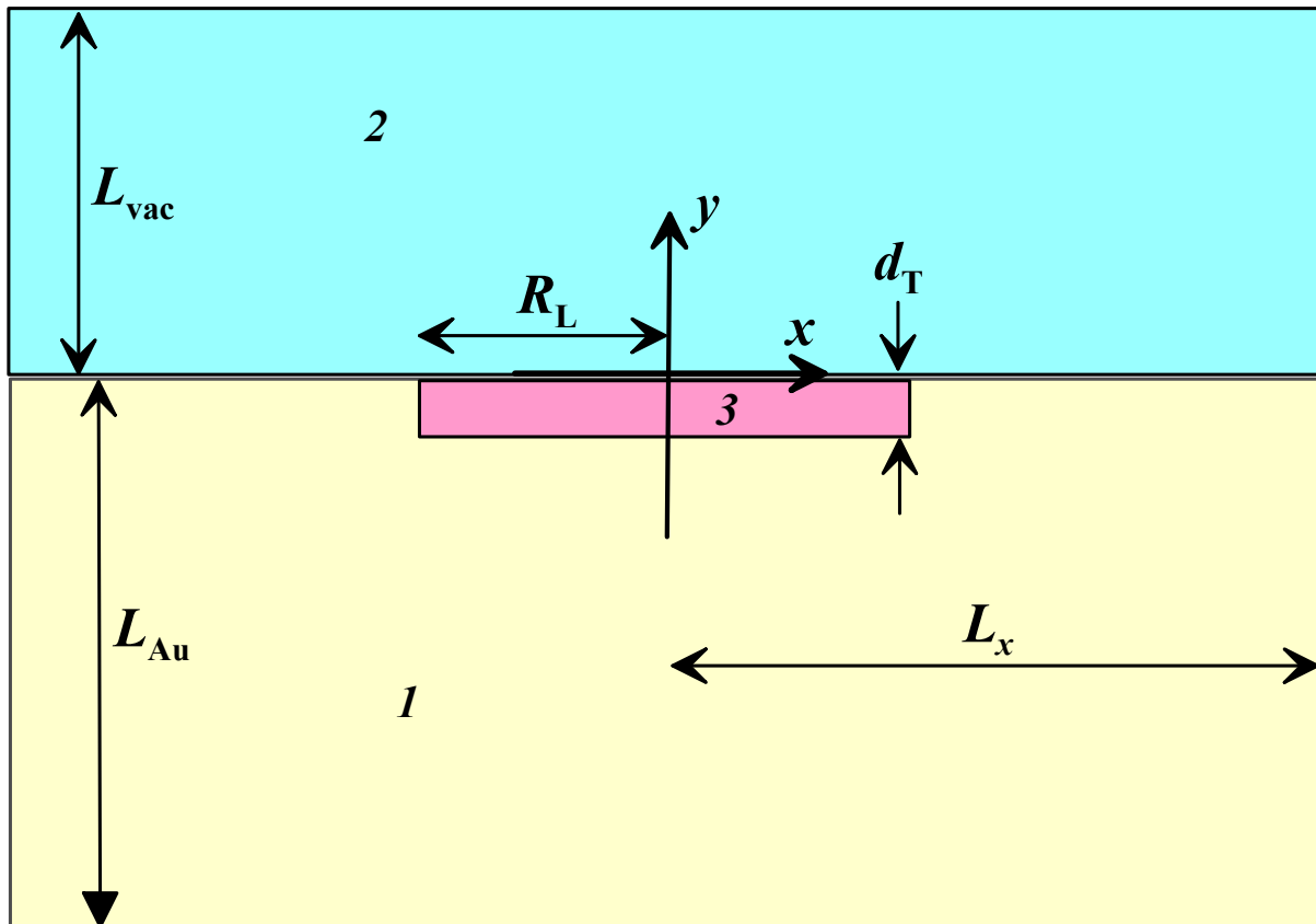
Figure 3. Diagram of the effect of an ultra-short laser pulse on the volumetric target (1). The half-width laser beam R_L passes through vacuum (2) and acts on the target. Ultrashort beam action in a hydrodynamic setting “instantly” creates a warmed up layer 3 with a thickness of d_T . The lengths of L_x and L_{Au} + L_{vac} determine the size of the calculated box.
